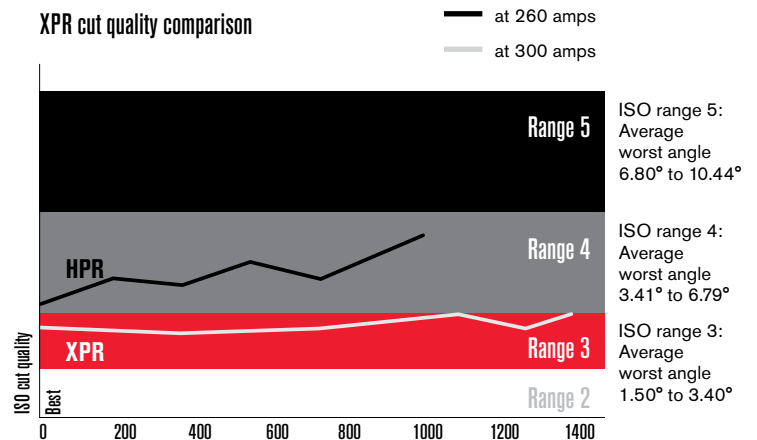
20-second cuts on mild steel
